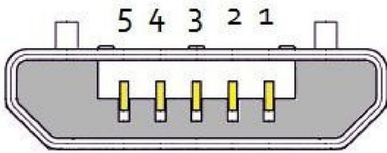
USB Micro-B
